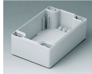
C1081201 Case shell 80, with tongue light grey RAL 7035 120x80x40mm
