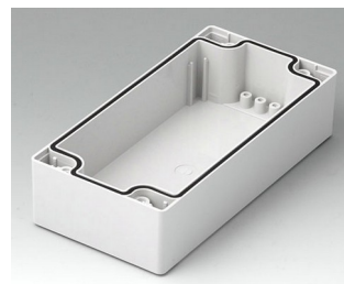
C2081601 Case shell 80, with groove light grey RAL 7035 160x80x40mm
