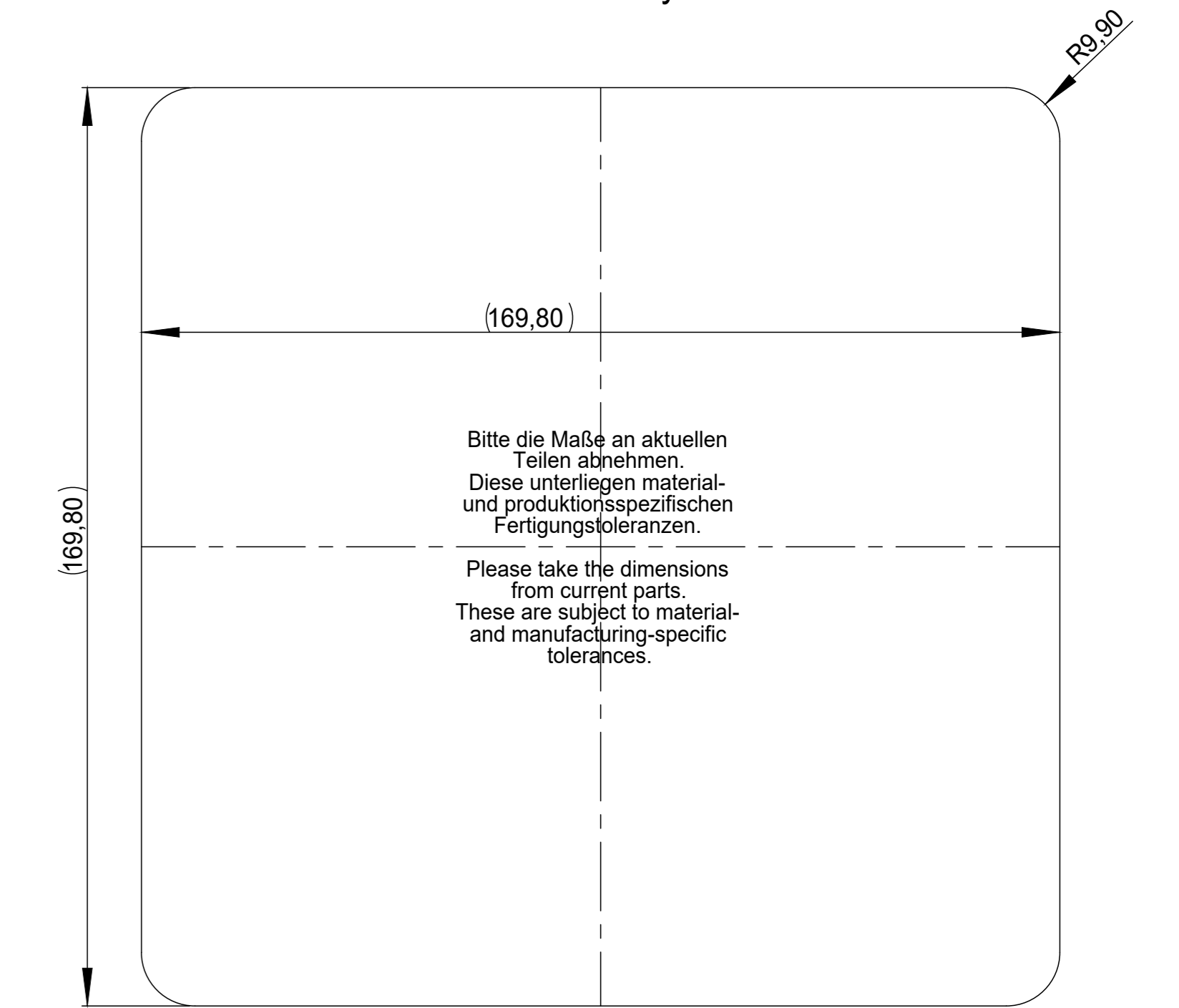
Folientastatur membrane keyboard
