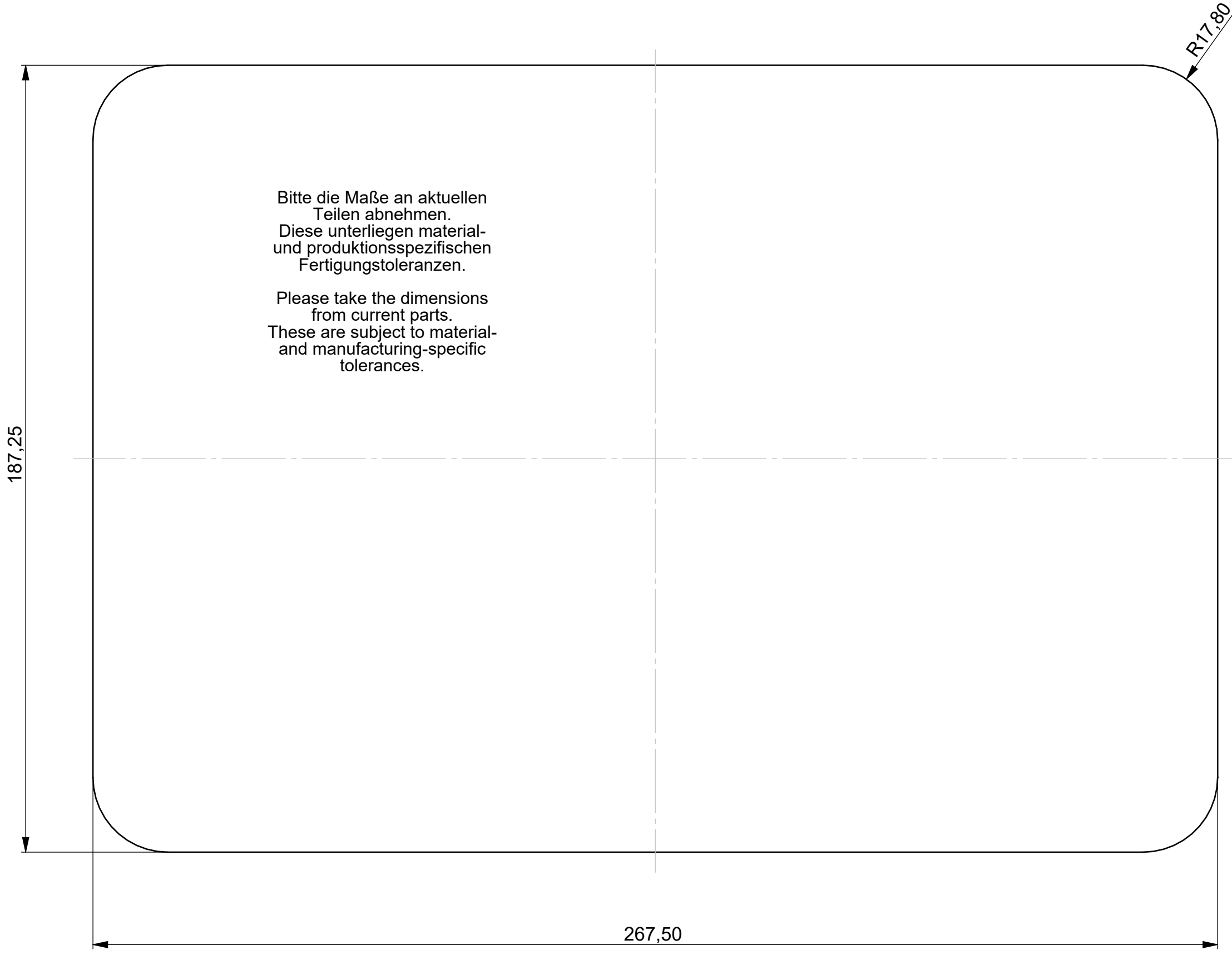
Folientastatur membrane keyboard
